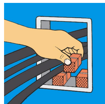
3 When packing the transit, ensure all the insert blocks have "E" marking facing the installer.
