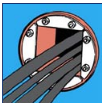
3 Pull the cables or pipes through, placing the largest at the bottom of the frame.
