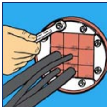
5 Tighten the bolts to compress and complete the seal. Approximately 10 to 12mm of thread should protrude on each bolt.
