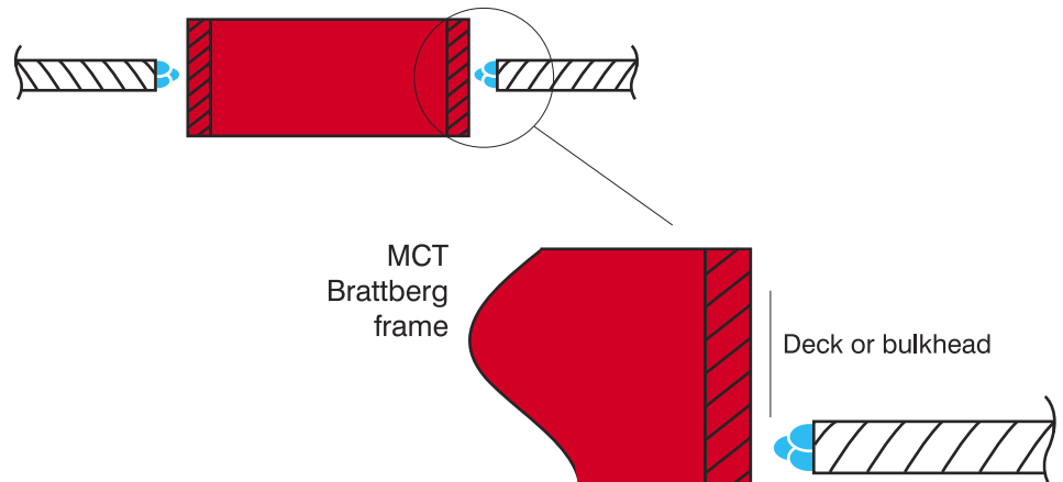
FIG 2: Build-up of fillet joint.
